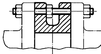
Figure 3 — Single flange or lugged wafer body
