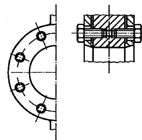
Figure 3d — Single-flange valve with internally threaded holes
