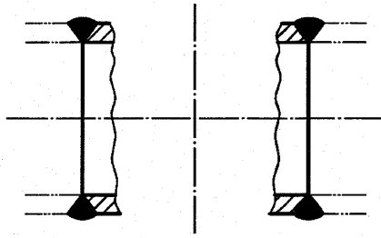
Figure 5 — Butt welding end body
