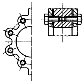
Figure 3c — Valve with lugs with internally threaded holes
